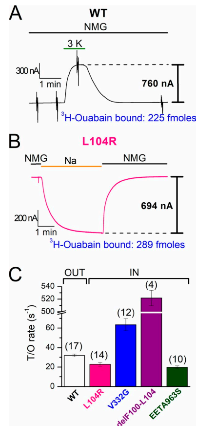
Figure 7. Turnover rates of wild-type and mutant human Na/K pumps. (A) Representative recording from an oocyte expressing wild-type pumps, held at -50 mV, in which application of 3 mM \text{K}^+ in \text{NMG}^+ induced outward current. (B) Representative recording from an oocyte expressing L104R pumps in which replacing \text{NMG}^+ with \text{Na}^+ solution induced inward current. The quantity of [^3\text{H}] ouabain bound to the oocytes in A and B is also indicated. (C) Bar graph showing mean turnover rates (moles of charge per second/moles of [^3\text{H}] ouabain bound; i.e., \text{s}^{-1} ) measured in individual oocytes, for the outward current (bracketed as “OUT”) in oocytes expressing wild type ( n = 17 ) and for the \text{Na}^+ -induced inward current (bracketed as “IN”) in oocytes expressing L104R, V332G, delF100-L104, and EETA963S. Measurements were performed 4–5 d after injection, except for delF100-L104, which was performed 3 d after injection because of large currents. Note the break along the y axis. The number of experiments is indicated in parentheses. Error bars represent SEM.
